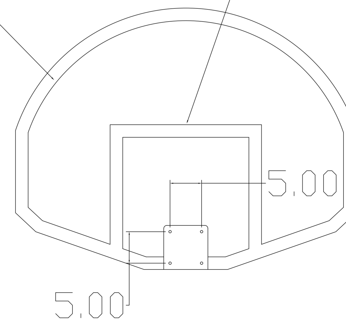
FRONT VIEW
